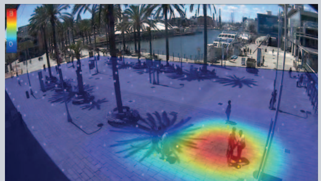
↑ HIGH/LOW DENSITY ESTIMATION
