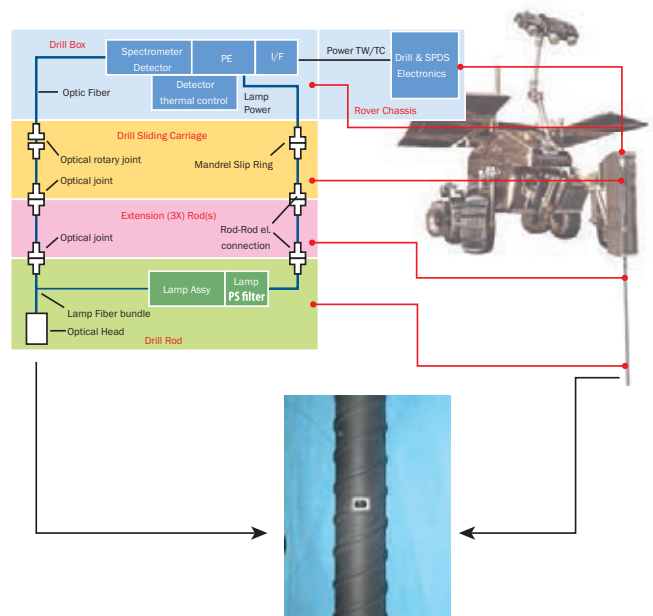
Ma_Miss connection schematics and optical observation port.
