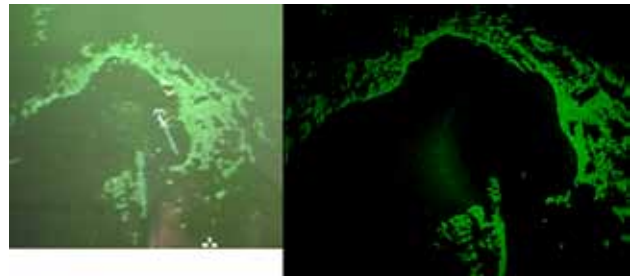
Comparison between a true Real Beam Ground Mapping (RBGM) radar image (left) and the corresponding real-time MARS simulation (right) using a non-coherent processing (Tyrrhenian sea and Coarse island).
