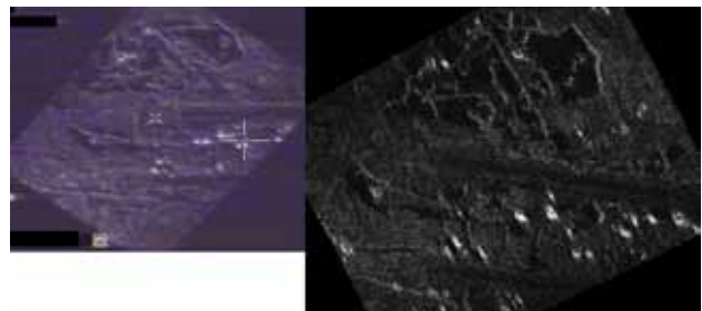
Comparison between a true Squinted Spotlight Doppler Beam Sharpening (SpDBS) image (left) and the corresponding real-time MARS simulation (right) using FFT processing (18 meters resolution on the Manching airport).
